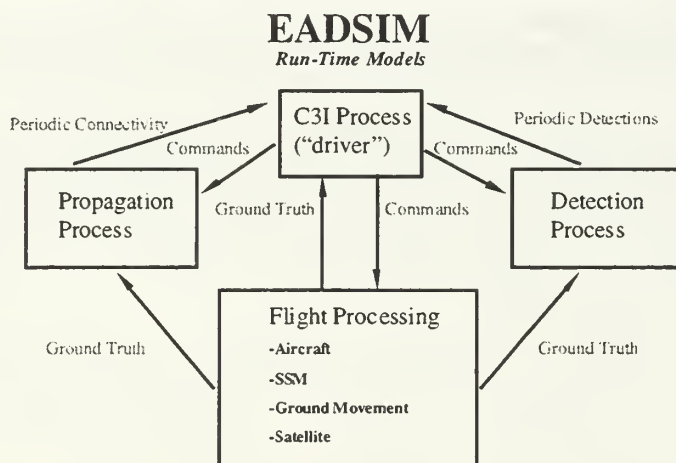
Figure 3. 3 EADSIM Interprocess Communication via Sockets. After Ref. [METH98]
